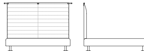
50044 + 50041 Giroletto + Testata imbottita alta Bed frame + High upholstered headboard cm 198 x 218 x h 146 in 78 x 85 7/8 x h 57 1/2 RETE - SLAT BASE cm 170 in 67
