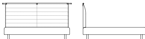
50054 + 50050 Giroletto + Testata imbottita bassa Bed frame + Low upholstered headboard cm 208 x 218 x h 111 in 81 7/8 x 85 7/8 x h 43 3/4 RETE - SLAT BASE cm 180 in 70 7/8
