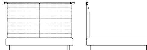
50054 + 50051 Giroletto + Testata imbottita alta Bed frame + High upholstered headboard cm 208 x 218 x h 146 in 81 7/8 x 85 7/8 x h 57 1/2 RETE - SLAT BASE cm 180 in 70 7/8
