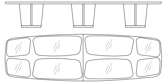
53141 Tavolo rettangolare in noce canaletto, inserti piano in vetro Rectangular table in walnut canaletto, top with glass inserts cm 450 x 134 x h 73 in 177 1/4 x 52 3/4 x h 28 3/4
