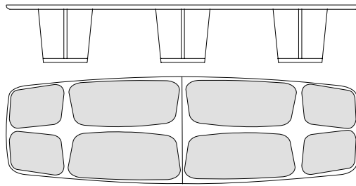
53140 Tavolo rettangolare in noce canaletto, inserti piano in pelle Rectangular table in walnut canaletto, top with leather inserts cm 450 x 134 x h 73 in 177 1/4 x 52 3/4 x h 28 3/4
