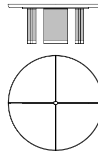
70007 Tavolo rotondo in acero gambe in cuoio, inserti sapelli Round table in maple saddle leather legs, sapele inserts Ø cm 180 x h 73 Ø in 70 7/8 x h 28 3/4
