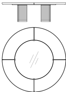
70003 Tavolo rotondo in acero gambe in cuoio piano girevole, inserti palissandro Round table in maple lazy susan saddle leather legs, rosewood inserts Ø cm 250 x h 73 Ø in 98 1/2 x h 28 3/4
