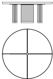
70016 Tavolo rotondo in acero gambe in cuoio, inserti marmo Round table in maple saddle leather legs, marble inserts Ø cm 180 x h 73 Ø in 70 7/8 x h 28 3/4
