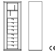
C 80052 Mobile girevole in noce canaletto con divisori e 8 cassetti Swivel cabinet in walnut canaletto with partitions and 8 drawers cm 69 x 52 x h 190 in 27 1/8 x 20 1/2 x h 74 7/8
