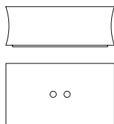
GA212G Scatola rettangolare con coperchio in marmo calacatta Rectangular box with calacatta marble cover cm 35 x 20 x h 12,5 in 13\frac{9}{8} x 7\frac{7}{8} x h 4\frac{7}{8}
