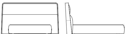
SF 59281 Letto testata alta Queen size Bed with high headboard Queen size cm 235 x 241 x h 130 in 92 ½ x 94 ¾ x h 51 ¼
