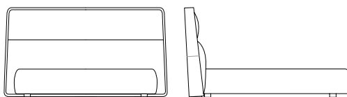
SF 59201 Letto testata alta Bed with high headboard cm 235 x 240 x h 130 in 92 ½ x 94 ½ x h 51 ¼
